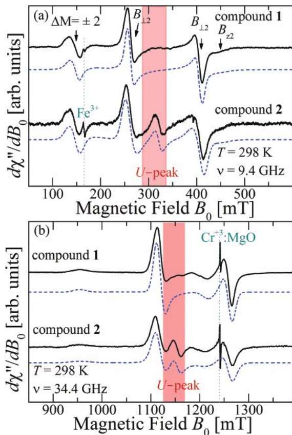
Fig. 10 Powder EPR spectra of compounds 1 and 2 collected at 298 K at (a) X- and (b) Q-bands. The source of the U-peaks emphasized with red backgrounds at \sim 300 and \sim 1125 mT in (a) and (b) is described in the text.
